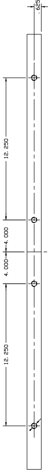
(2) .438-14-UNC-2B EACH PANEL
