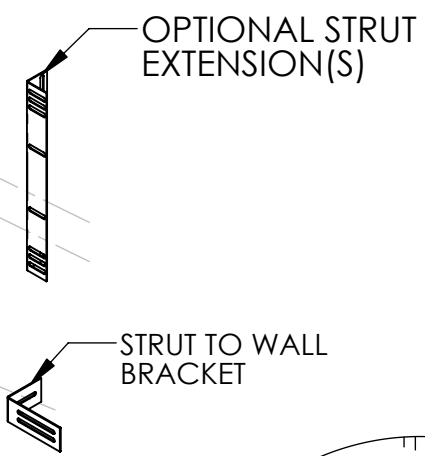
DOOR TOP CHANNEL DETAIL
