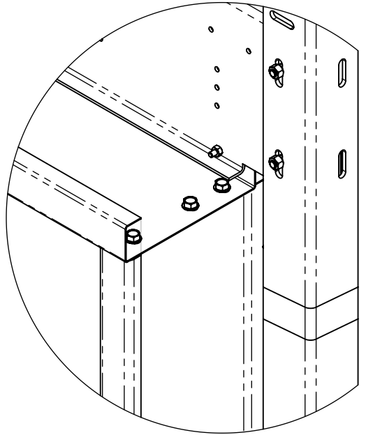
DETAIL B SCALE 1 : 6
