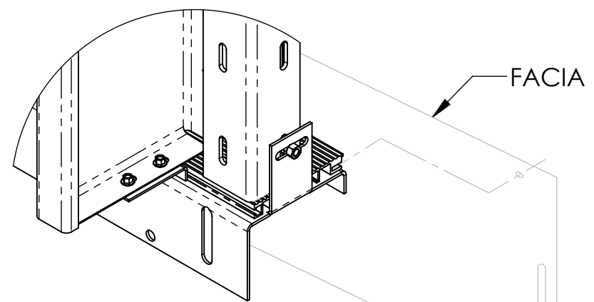
DETAIL D SCALE 1 : 6
